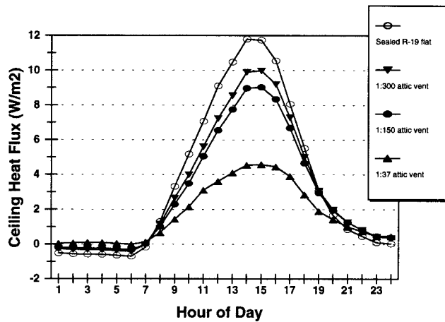
Figure 3 Orlando peak day ceiling heat flux for the sealed attic, and normal to very large ventilation areas, all with R-19 flat ceiling insulation.
