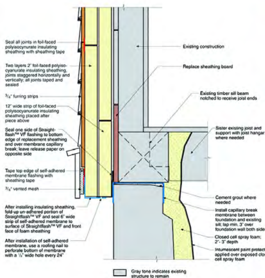
Figure 7 Sill detail, including air barrier transition wrapped to front of foam, and capillary break over foundation (left); existing sill beam, showing long-term moisture damage (right).
