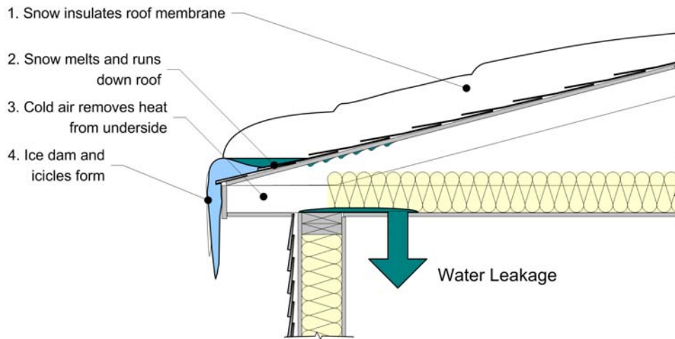
Figure 1: Ice Dam at a Typical Roof
