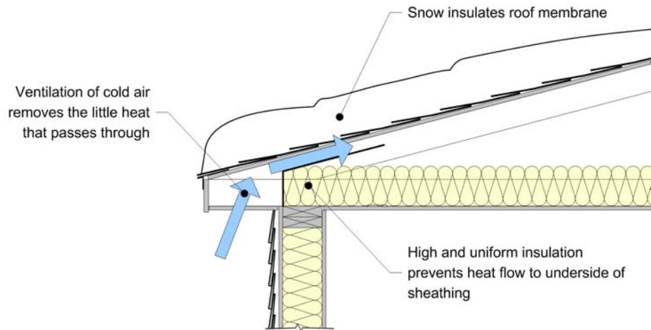
Figure 3: Solutions to Poor Insulation
