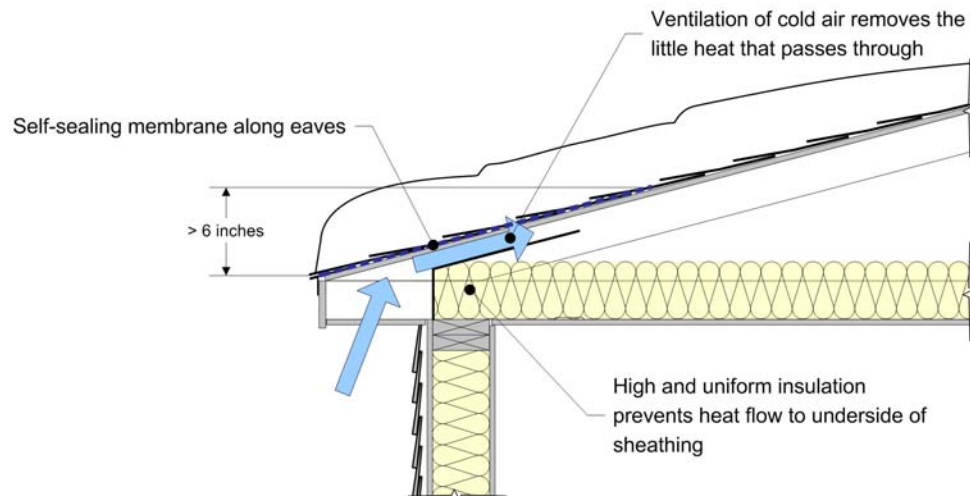
Figure 6: Waterproof "eaves-starter" or "peel and stick"
