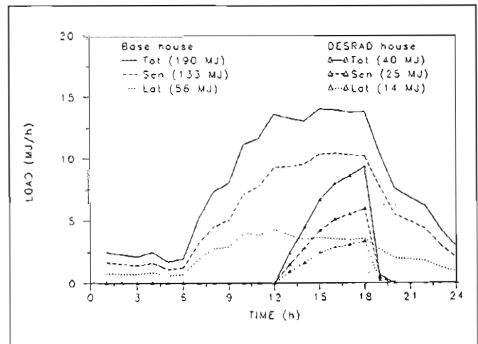
Fig. 2 Comparison of summer day cooling load requirements for base and DESRAD houses in Atlanta, Georgia
