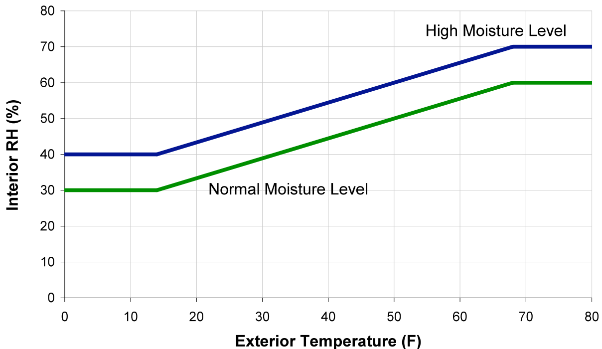
Figure 4: EuroNorm Standard 15026 Model for Interior RH Levels
