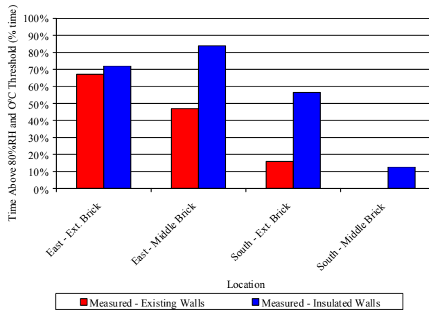
FIGURE 10: MEASURED TIME ABOVE CORROSION THRESHOLDS IN INSULATED AND EXISTING WALLS Insulated walls have significantly more time above corrosion thresholds than existing walls, increasing risks for embedded steel corrosion in insulated walls.
