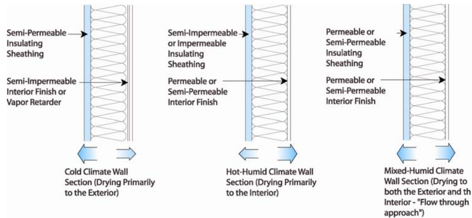
Figure 2. Vapor Diffusion Profiles
