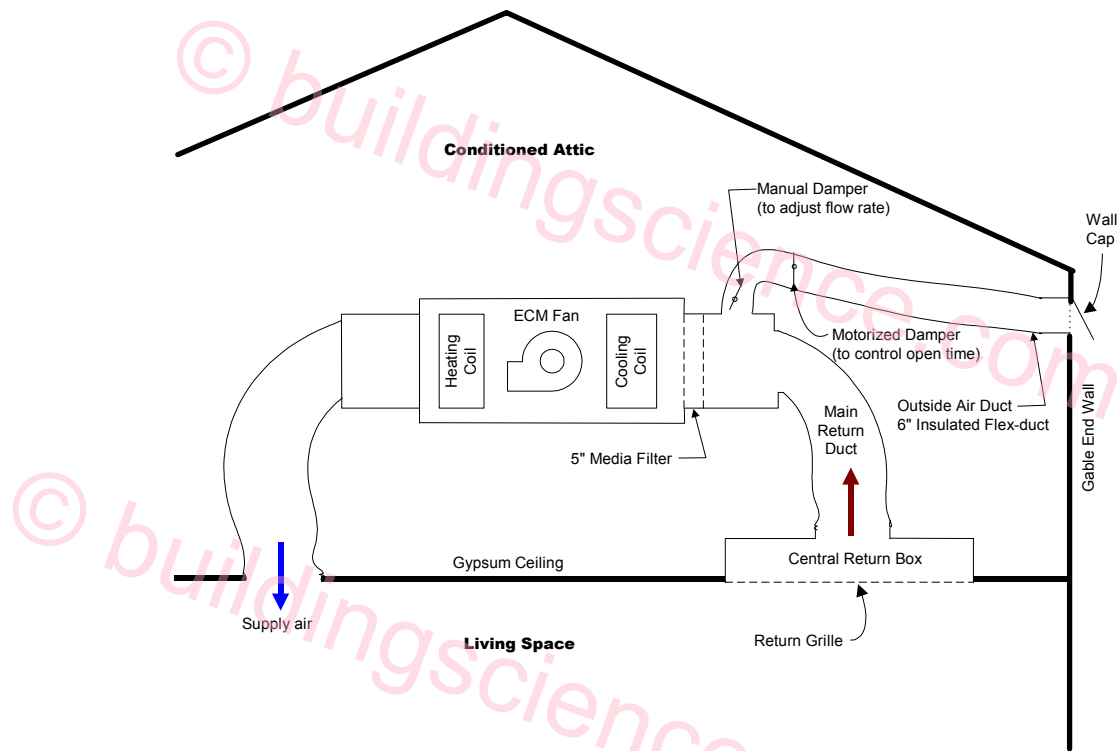
Figure A-6b. Schematic of two-stage compressor with ECM fan and Thermidistat system; evaporator section located in conditioned attic; ventilation is by central-fan-integrated supply; enhanced dehumidification was expected by long runtime with first stage compressor, slower fan speeds, and cooling below the setpoint as orchestrated by the Thermidistat control
