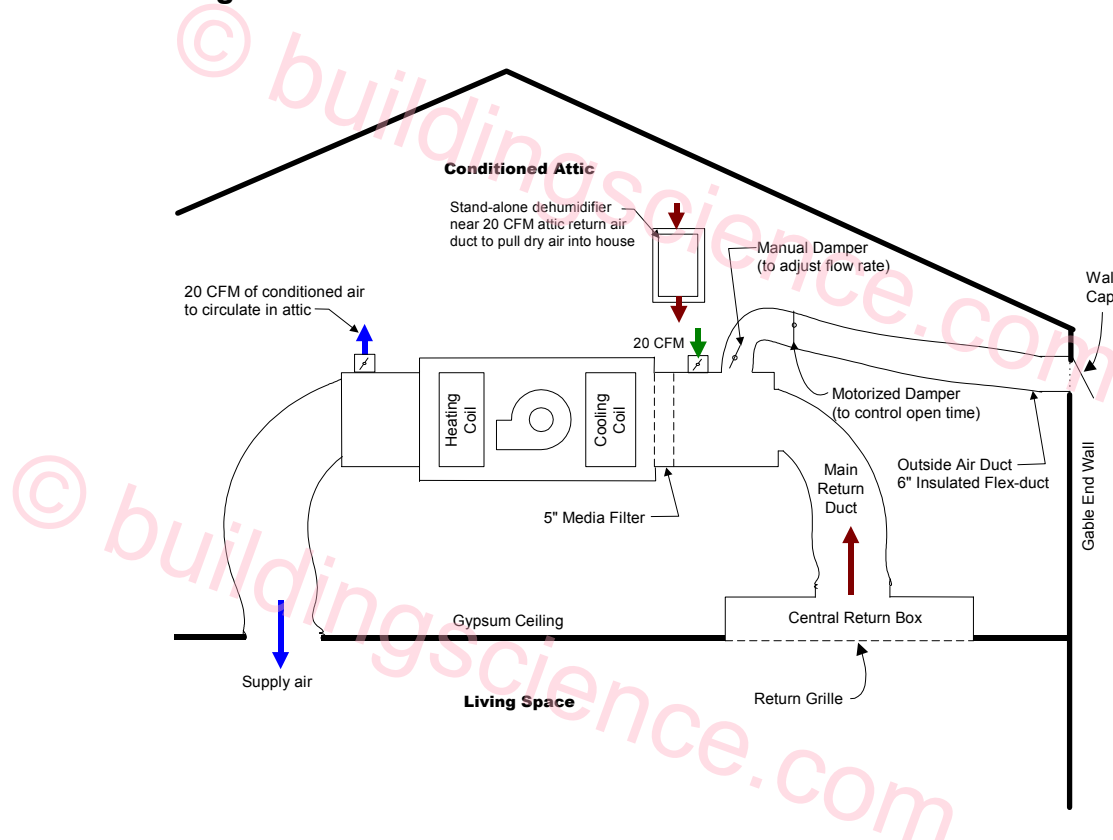
Figure A-2b. Schematic of stand-alone dehumidifier in conditioned attic system; dry air is delivered to the house via a small attic return duct placed near dehumidifier; ventilation is by central-fan-integrated supply as in all the standard Building America houses
