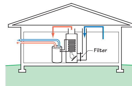
Sealed combustion power vented water heater located in the conditioned space (in utility room with air handler); water heater flue gases exhausted to exterior using fan; combustion air supplied directly to water heater from exterior via duct.
