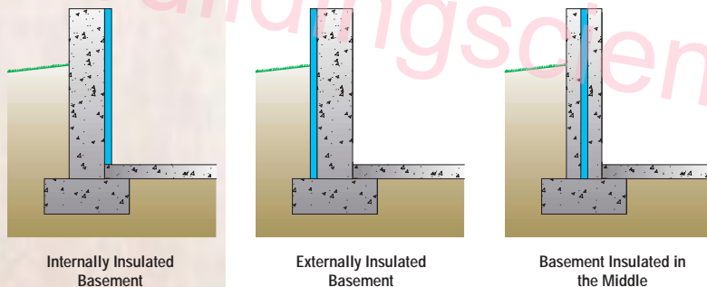
Figure 1 Basement insulation locations
