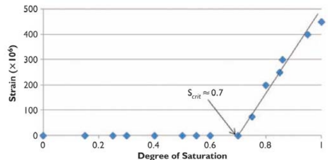
Figure 1: Critical Degree of Saturation —This is measured as a percentage of the vacuum saturation of the brick. From Mensinga, P. 2009. "Determining the Critical Degree of Saturation of Brick Using Frost Dilatometry." Master of Applied Science in Civil Engineering Thesis, University of Waterloo, Waterloo, ON, Canada. This youngster is on to something here. Memo to self: keep an eye on him, he looks destined for great things.
