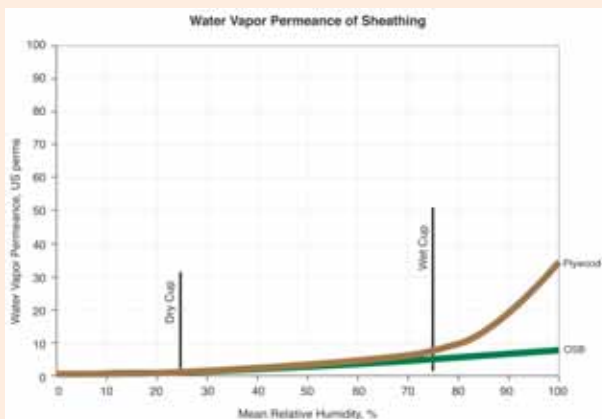
Figure A: Notice the difference between the wet cup and dry cup tests. And the huge difference at the end of the scale when things are really wet. Plywood passes moisture better than OSB, redistributes moisture better than OSB and dries much faster when it gets wet. This graph helps explain why. But, with an air gap we can compensate for this difference and make OSB the future standard for structural sheathings.
