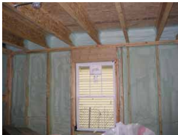
Photograph 5: High-Density Spray Foam Cavity Insulation —High tech and low perm. Great air sealing, great thermal performance, great structural strength. Does not allow for any appreciable inward drying of the exterior sheathing.
