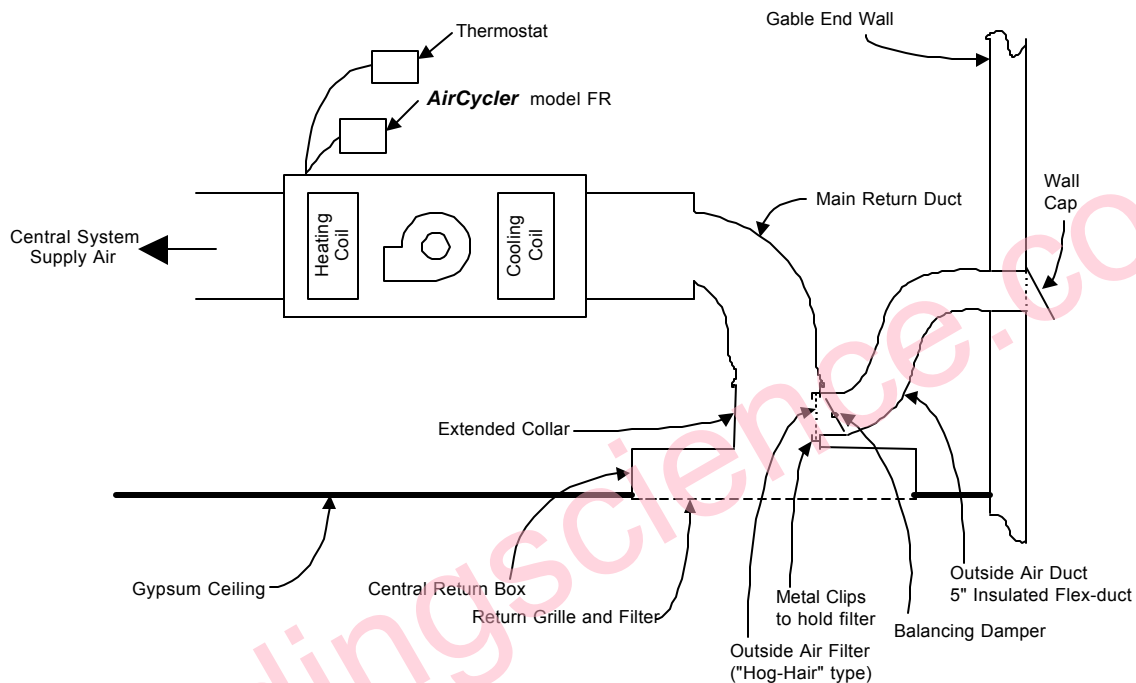
Figure 2 Central-fan-integrated supply ventilation; outside air duct into extended collar
